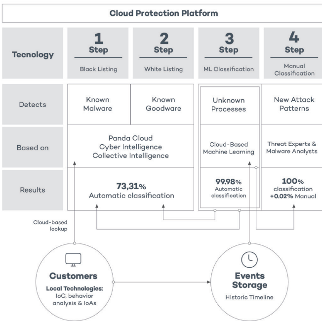
Figure 2: Workflow of the managed cloud classification service
